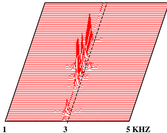
Figure 11 Waterfall Spectra from the Simulated Bird Song
